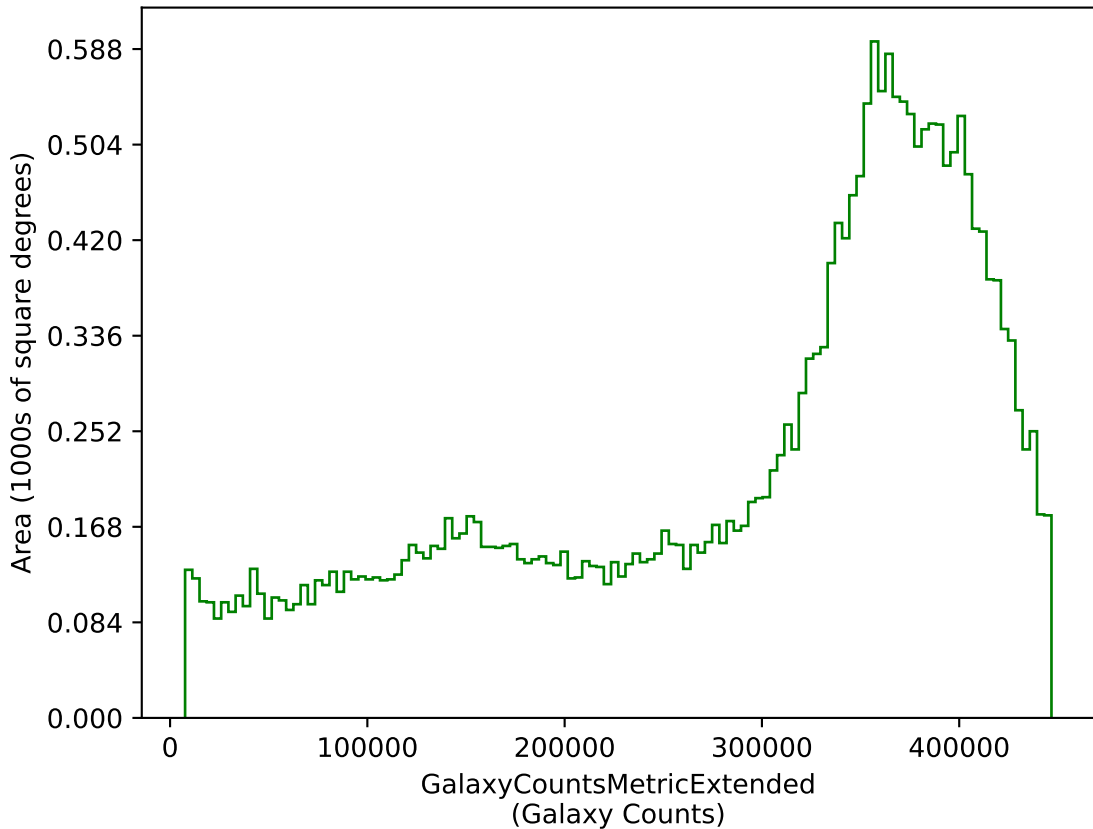
too_5_4v3.4_10yrs g: GalaxyCountsMetricExtended
