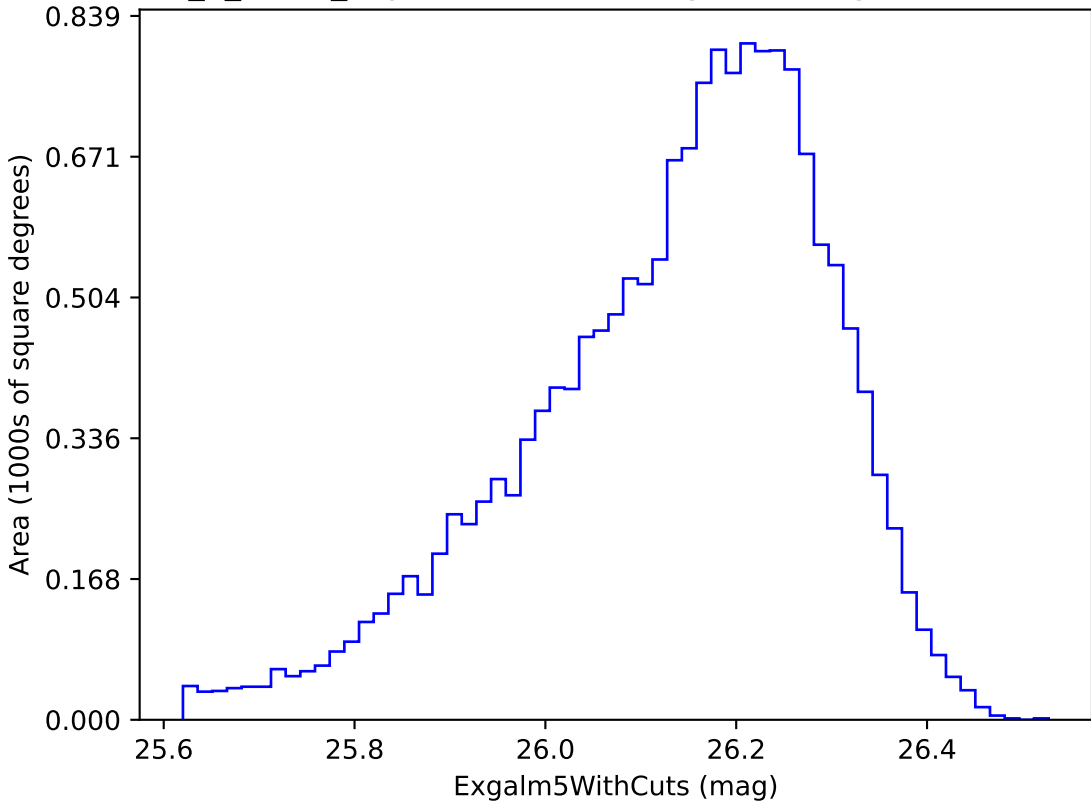
too_5_4v3.4_10yrs i band non-DD year 6: ExgalM5WithCuts
