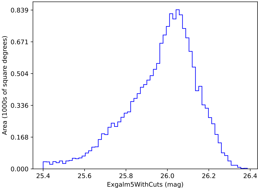
too_5_4v3.4_10yrs i band non-DD year 4: ExgalM5WithCuts
