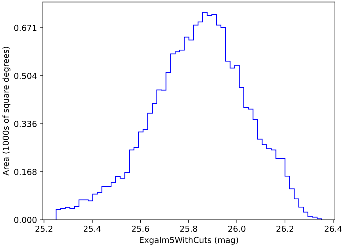
too_5_4v3.4_10yrs i band non-DD year 3: ExgalM5WithCuts
