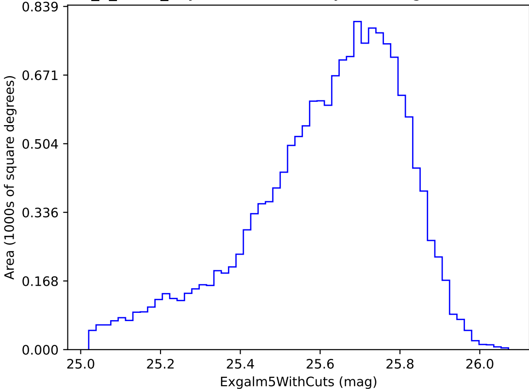
too_5_4v3.4_10yrs i band non-DD year 2: ExgalM5WithCuts
