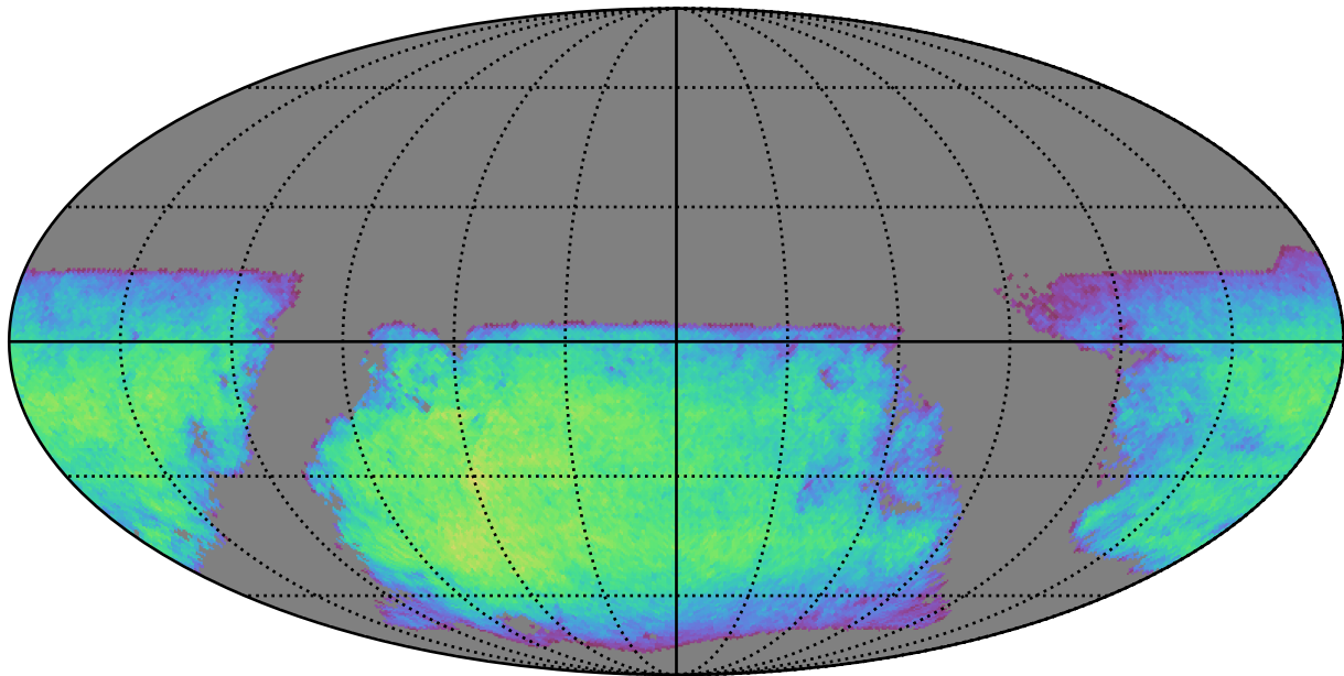
too_5_4v3.4_10yrs i band non-DD year 10: ExgalM5WithCuts
