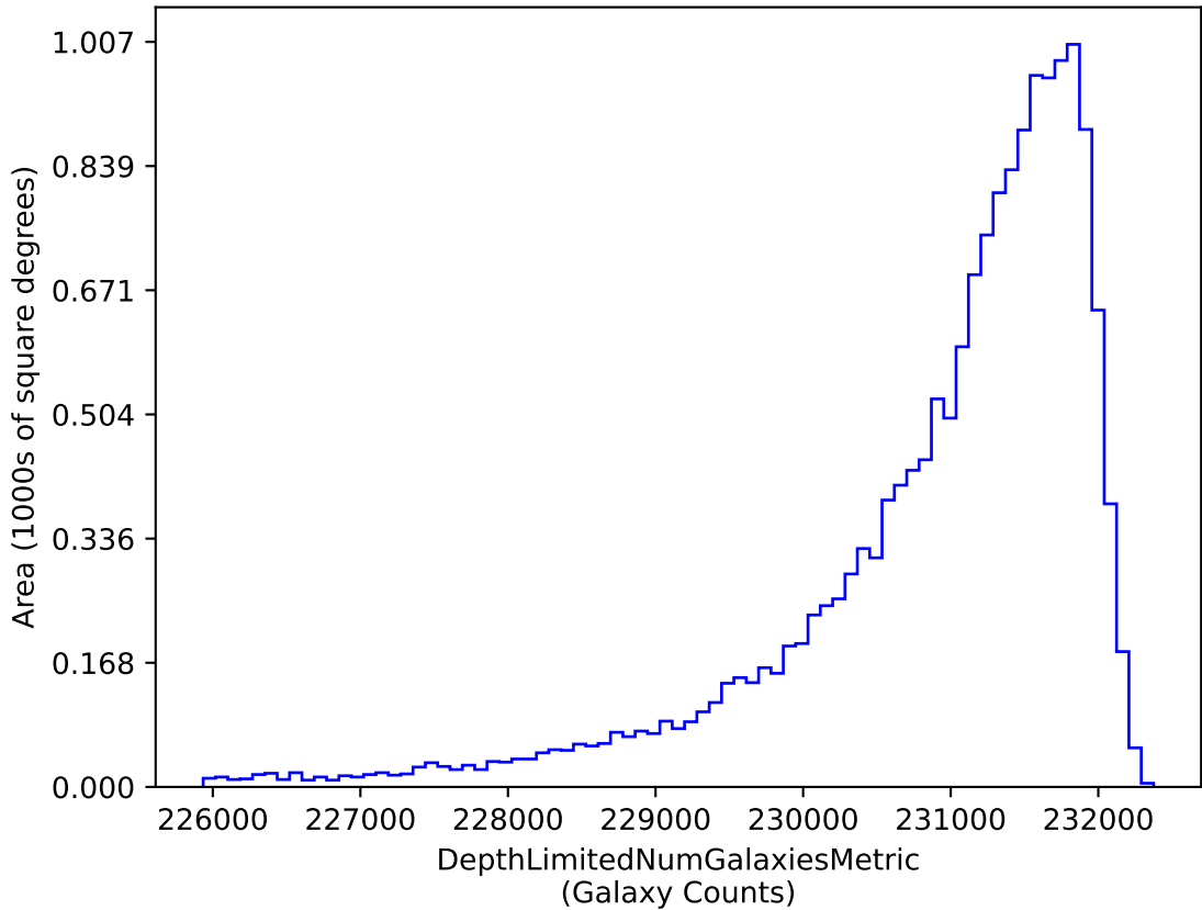
too_5_4v3.4_10yrs i band galaxies non-DD: DepthLimitedNumGalaxiesMetric
