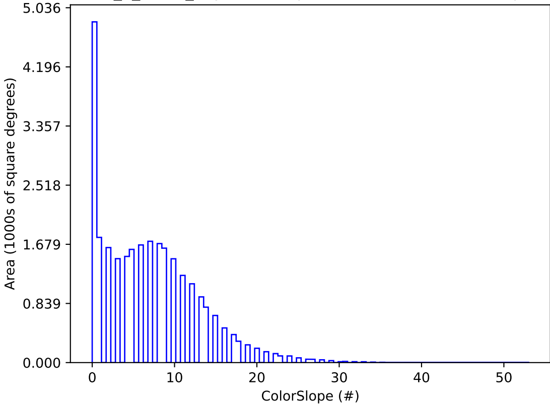
too_5_4v3.4_10yrs visitExposureTime > 19: ColorSlope
