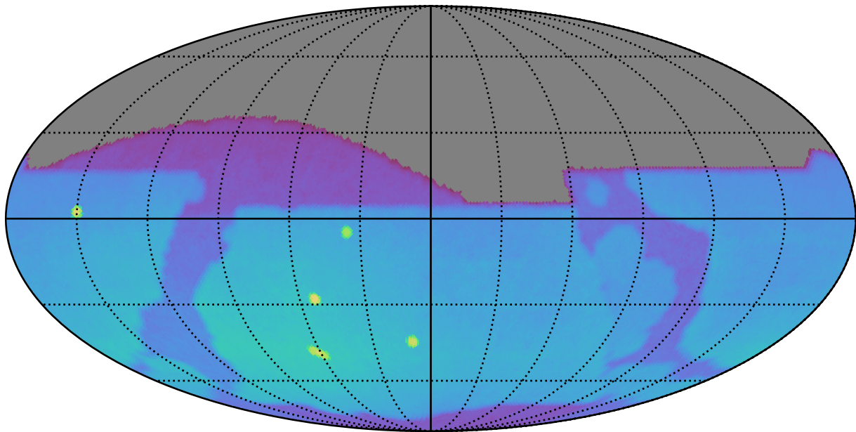
too_5_4v3.4_10yrs : Brown Dwarf, L4
