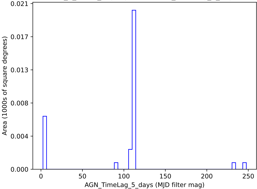
too_5_4v3.4_10yrs y band: AGN_TimeLag_5_days
