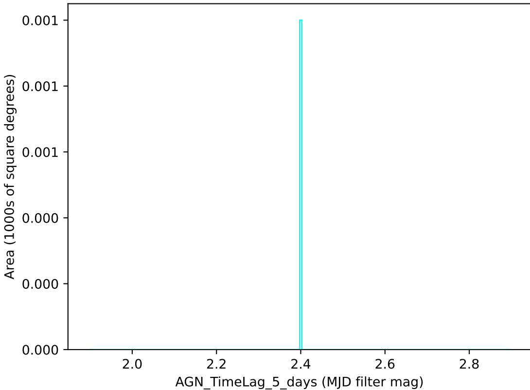
too_5_4v3.4_10yrs u band: AGN_TimeLag_5_days
