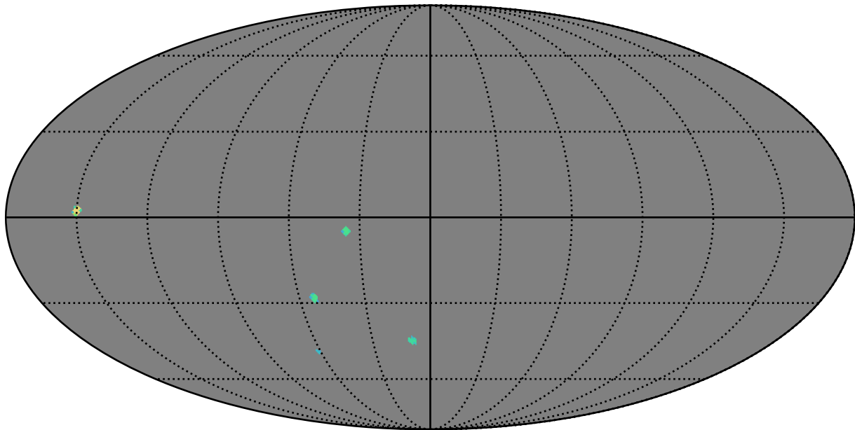
too_5_4v3.4_10yrs r band: AGN_TimeLag_5_days
