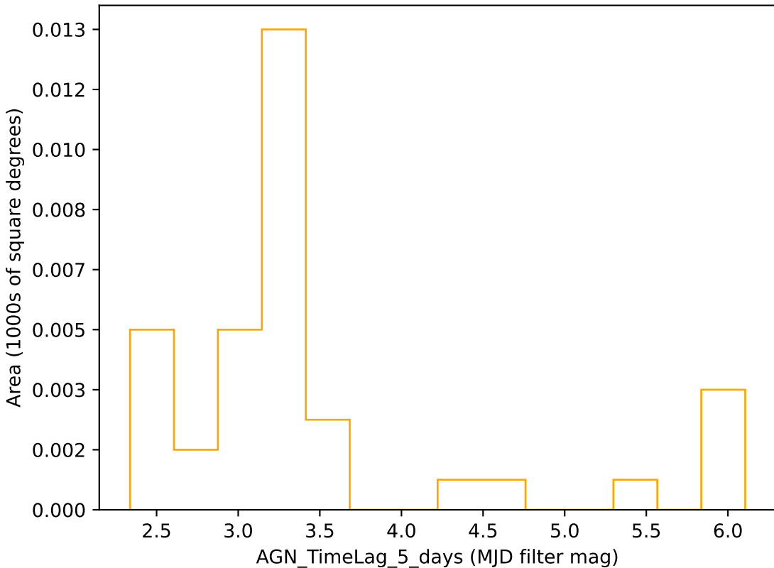
too_5_4v3.4_10yrs r band: AGN_TimeLag_5_days
