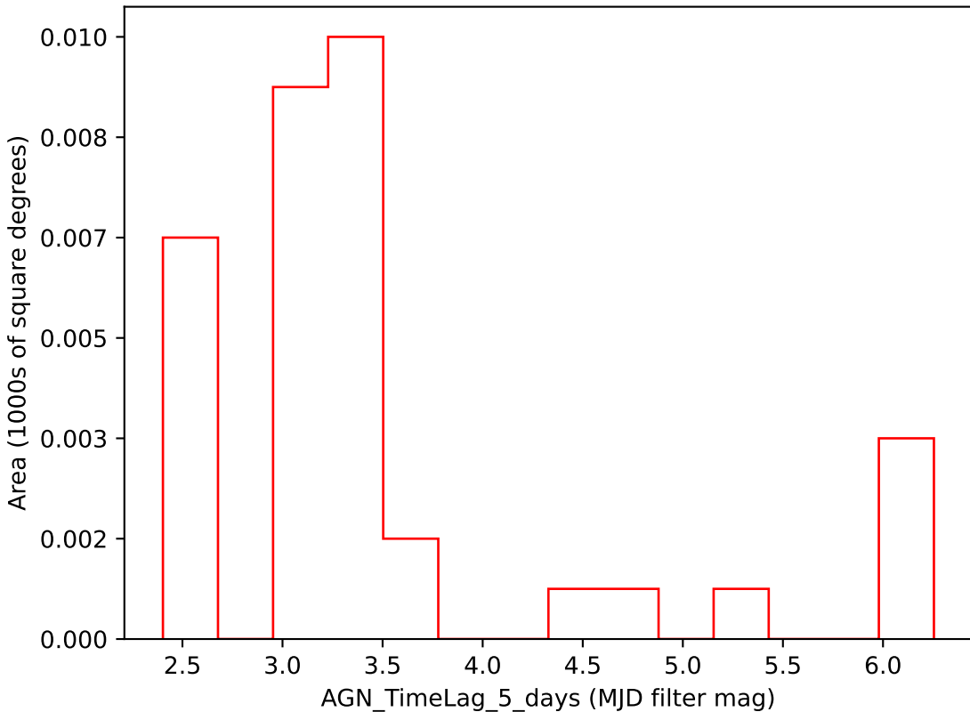
too_5_4v3.4_10yrs i band: AGN_TimeLag_5_days
