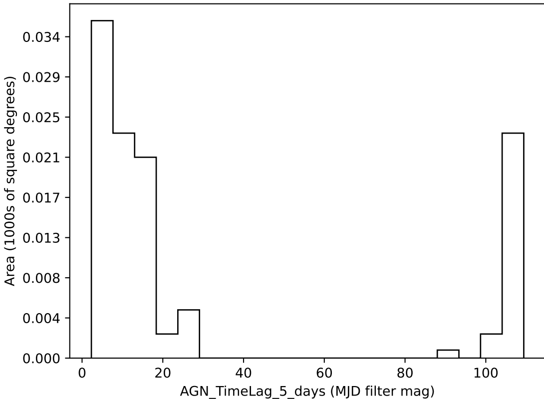
too_5_4v3.4_10yrs all bands: AGN_TimeLag_5_days
