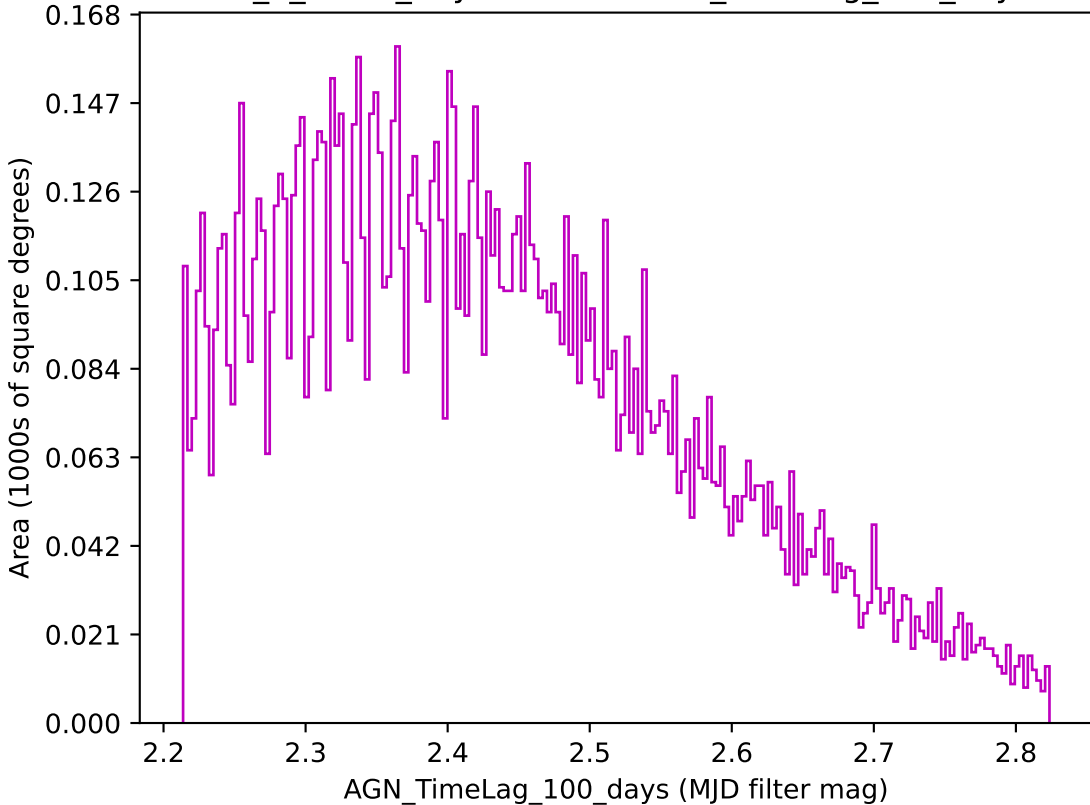
too_5_4v3.4_10yrs z band: AGN_TimeLag_100_days
