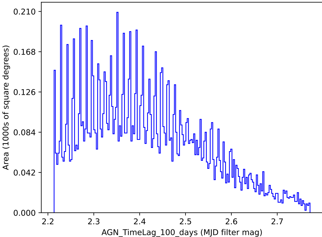
too_5_4v3.4_10yrs y band: AGN_TimeLag_100_days
