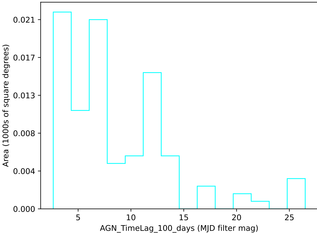
too_5_4v3.4_10yrs u band: AGN_TimeLag_100_days
