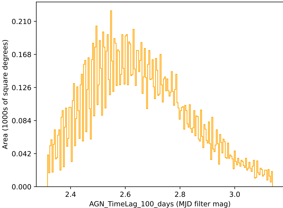
too_5_4v3.4_10yrs r band: AGN_TimeLag_100_days
