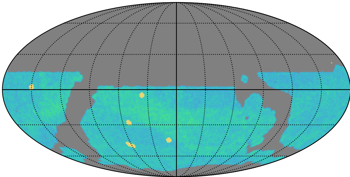
too_5_4v3.4_10yrs i band: AGN_TimeLag_100_days
