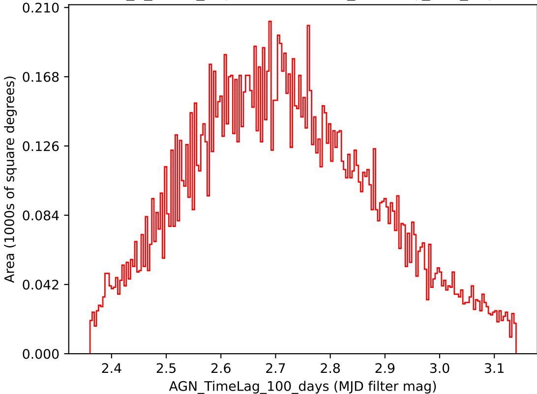
too_5_4v3.4_10yrs i band: AGN_TimeLag_100_days
