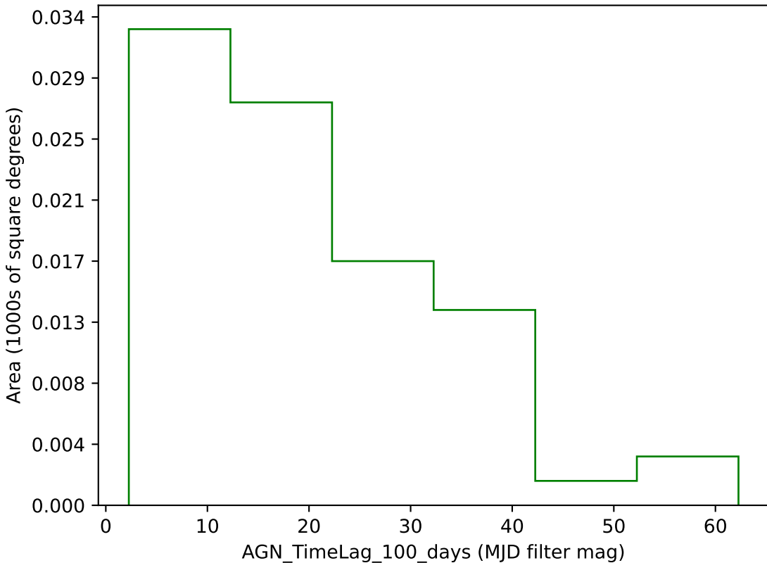
too_5_4v3.4_10yrs g band: AGN_TimeLag_100_days
