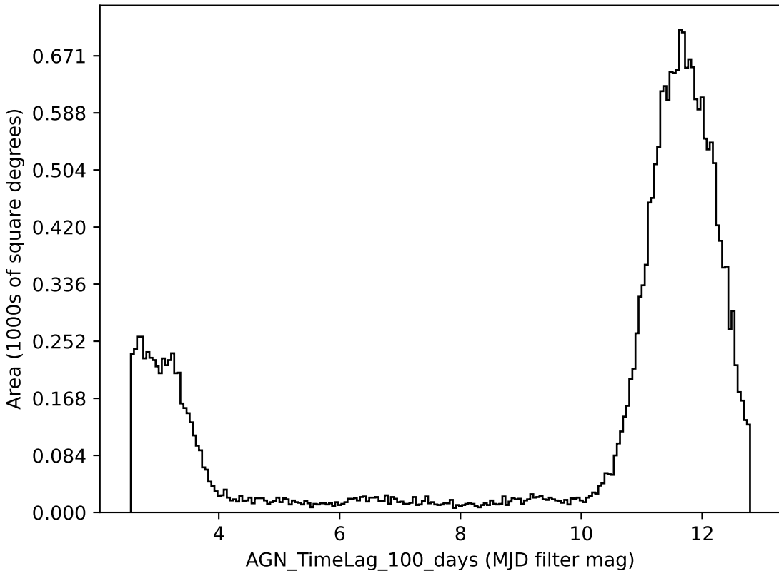
too_5_4v3.4_10yrs all bands: AGN_TimeLag_100_days
