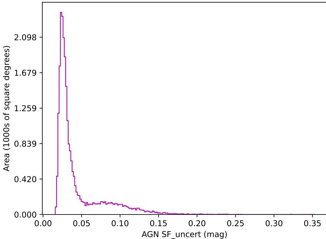
too_5_4v3.4_10yrs z band: AGN SF_uncert
