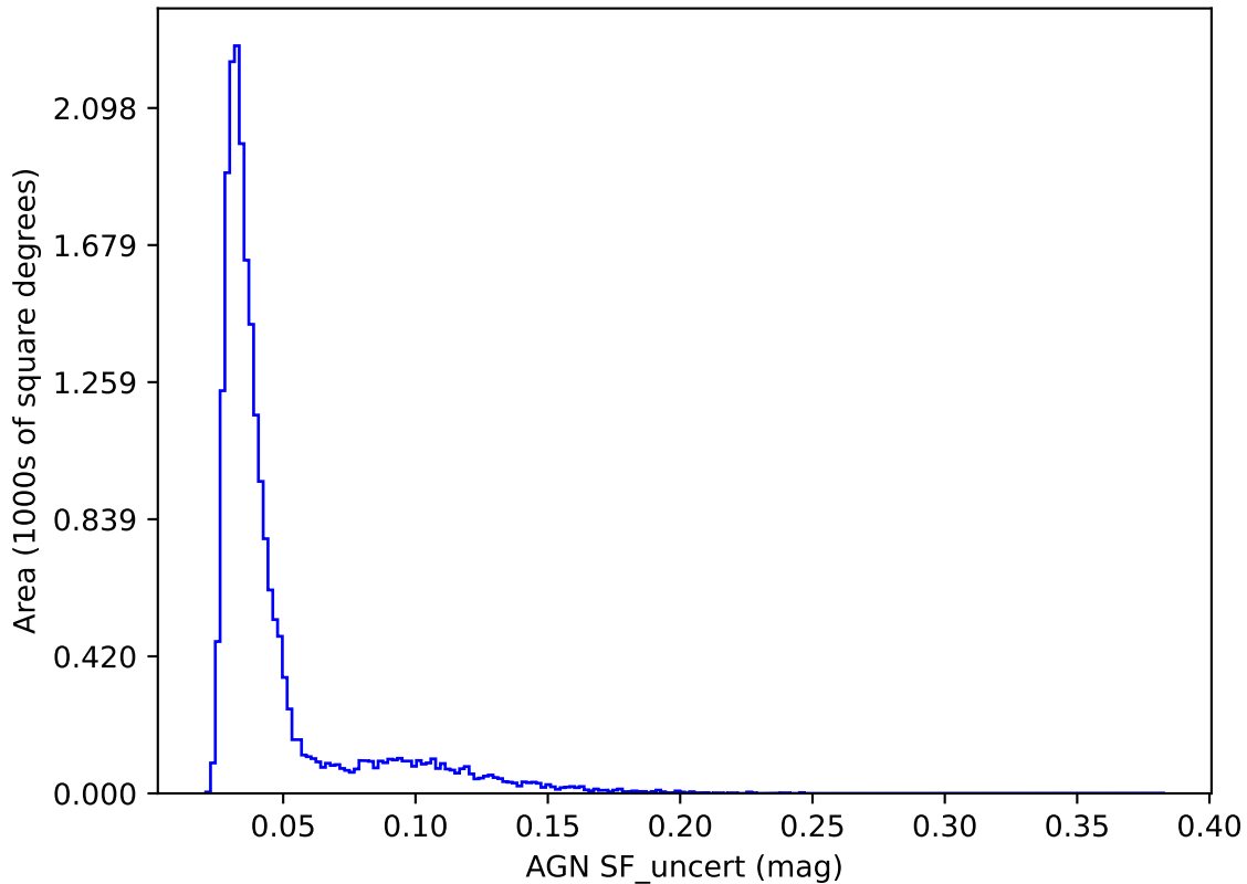
too_5_4v3.4_10yrs y band: AGN SF_uncert
