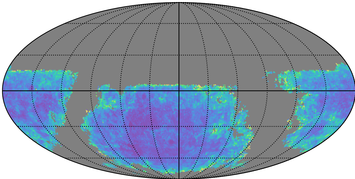
too_5_4v3.4_10yrs u band: AGN SF_uncert
