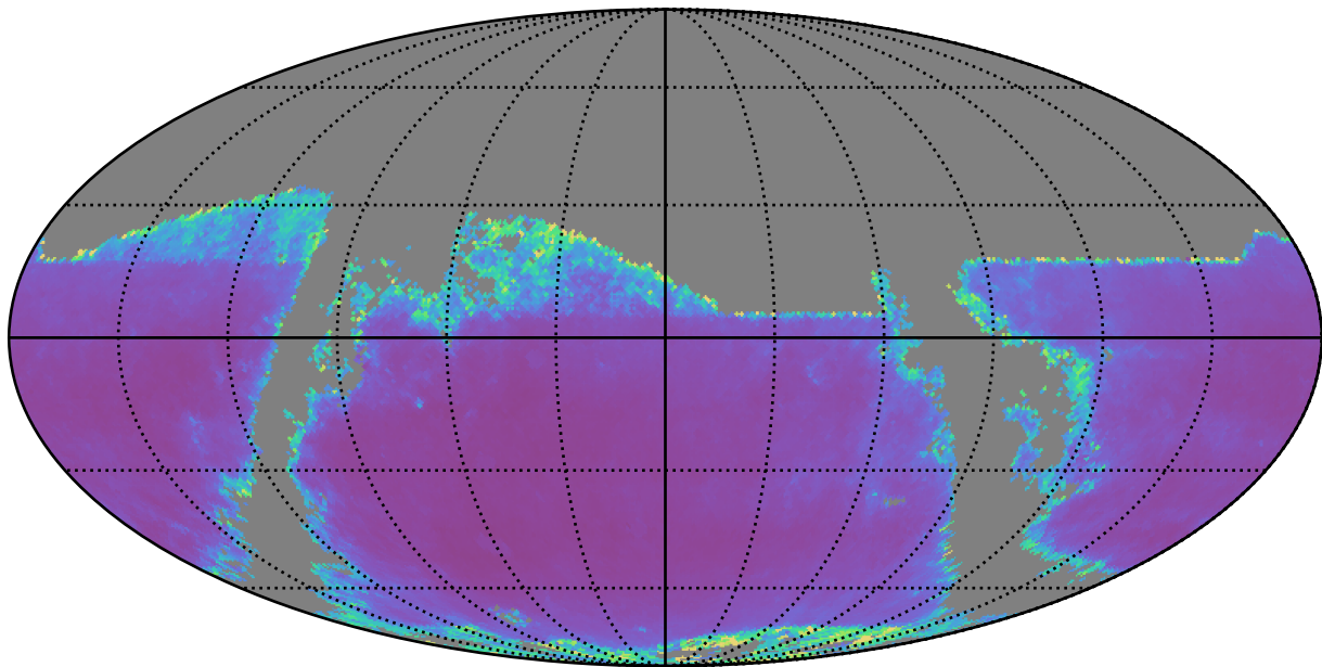
too_5_4v3.4_10yrs r band: AGN SF_uncert
