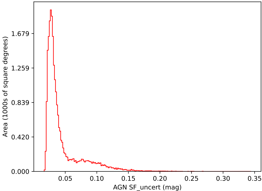
too_5_4v3.4_10yrs i band: AGN SF_uncert
