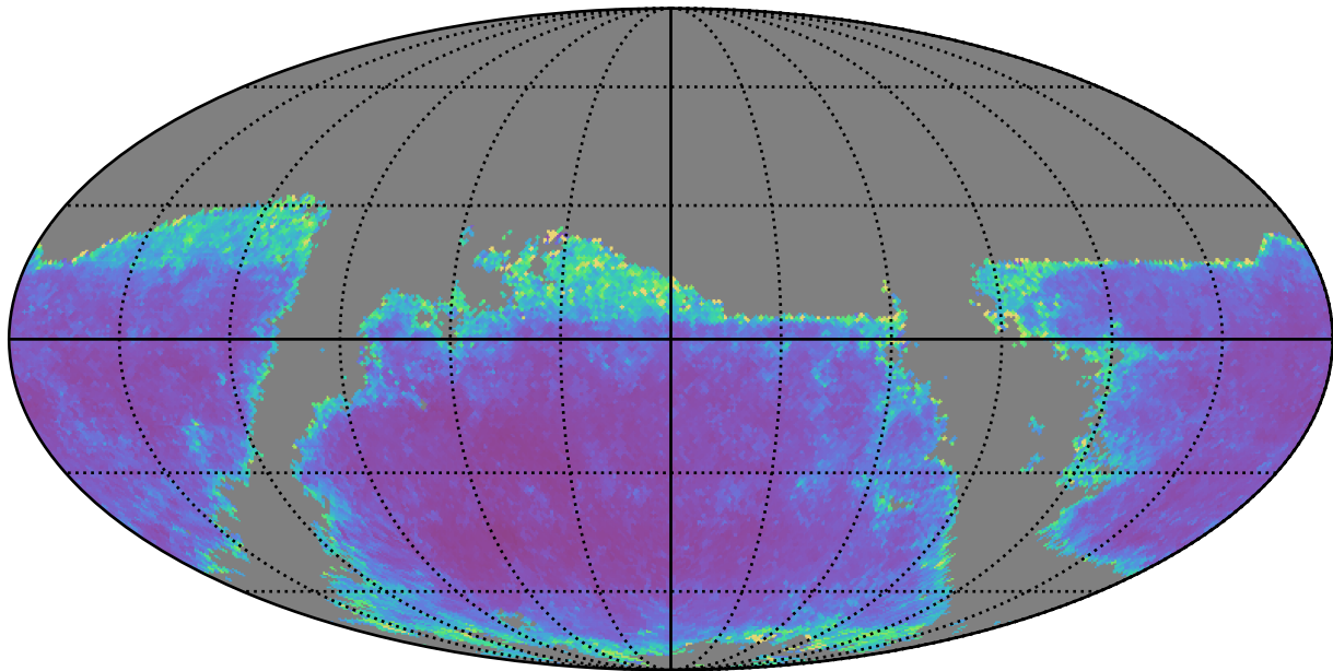
too_5_4v3.4_10yrs g band: AGN SF_uncert
