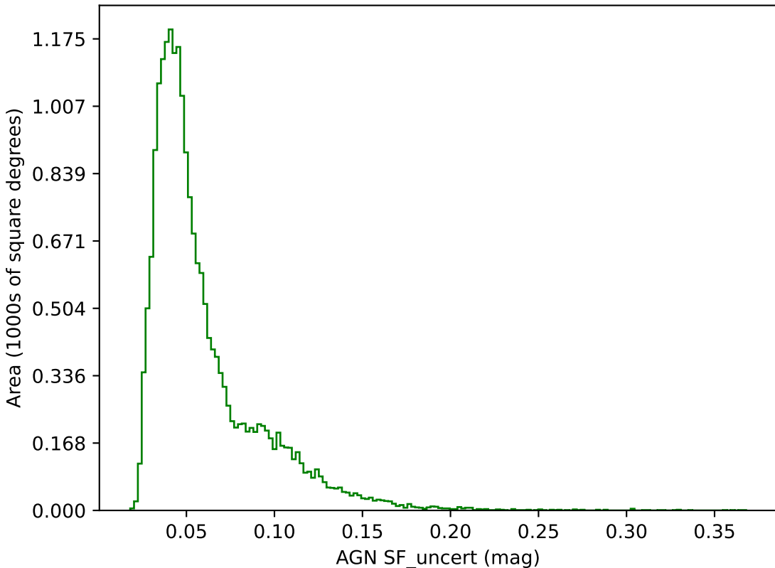
too_5_4v3.4_10yrs g band: AGN SF_uncert
