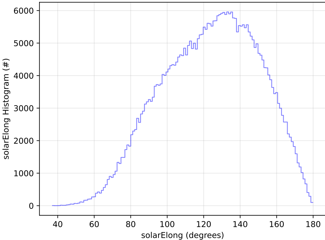
too_5_4v3.4_10yrs WFD y band: solarElong Histogram
