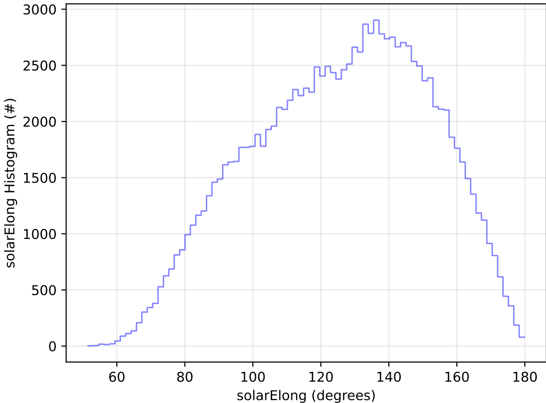
too_5_4v3.4_10yrs WFD u band: solarElong Histogram
