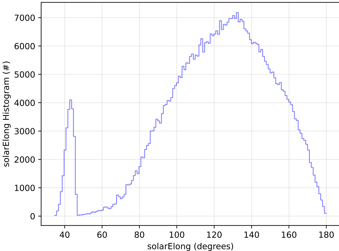
too_5_4v3.4_10yrs WFD i band: solarElong Histogram
