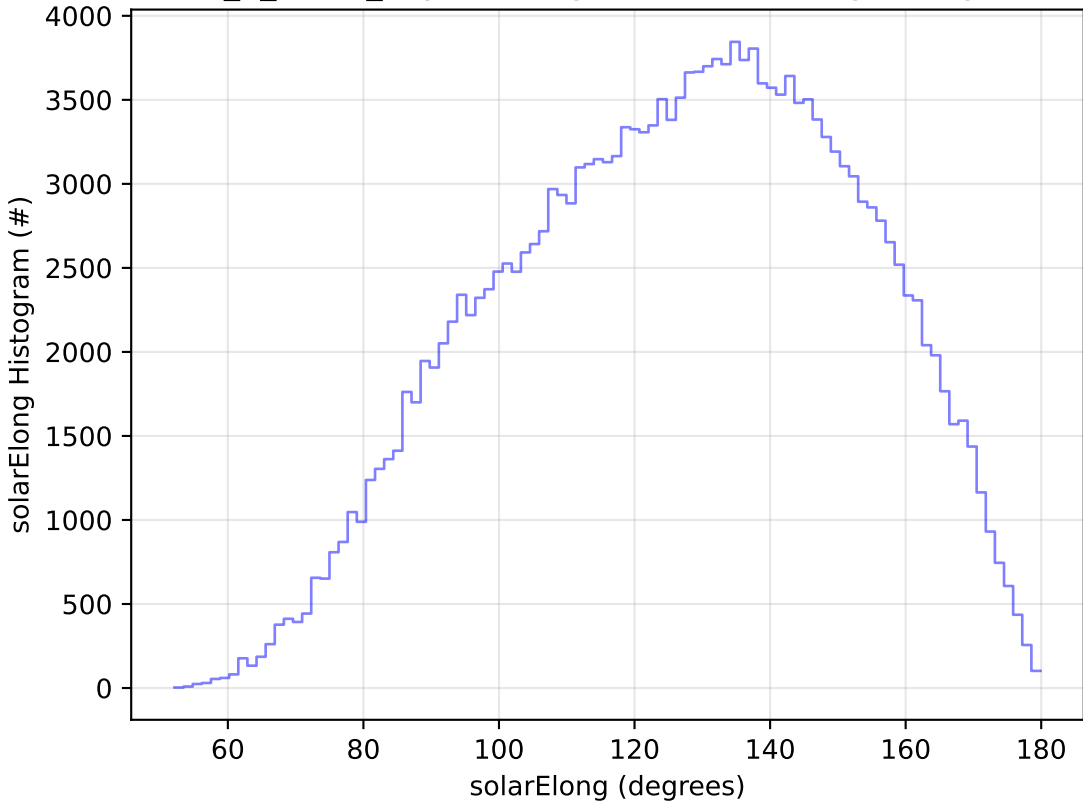
too_5_4v3.4_10yrs WFD g band: solarElong Histogram
