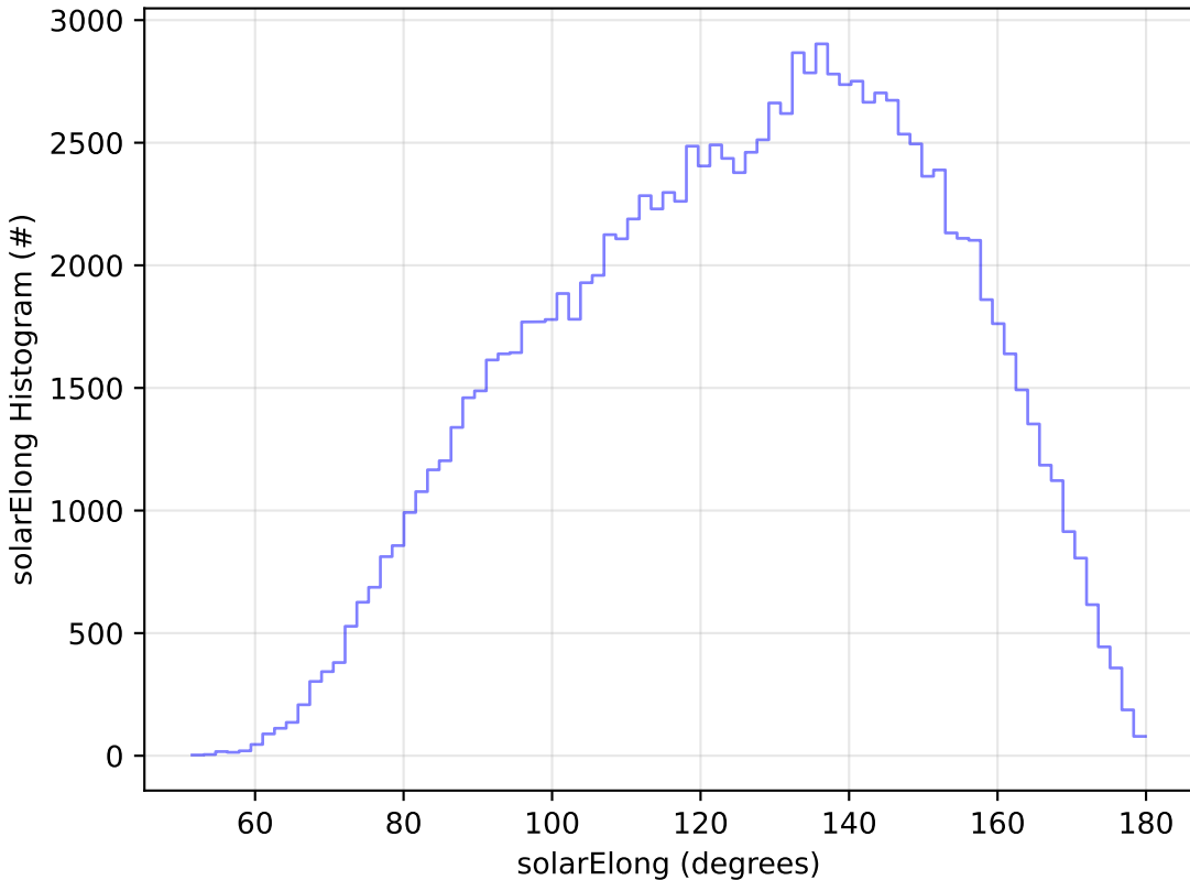
too_5_4v3.4_10yrs All sky u band: solarElong Histogram
