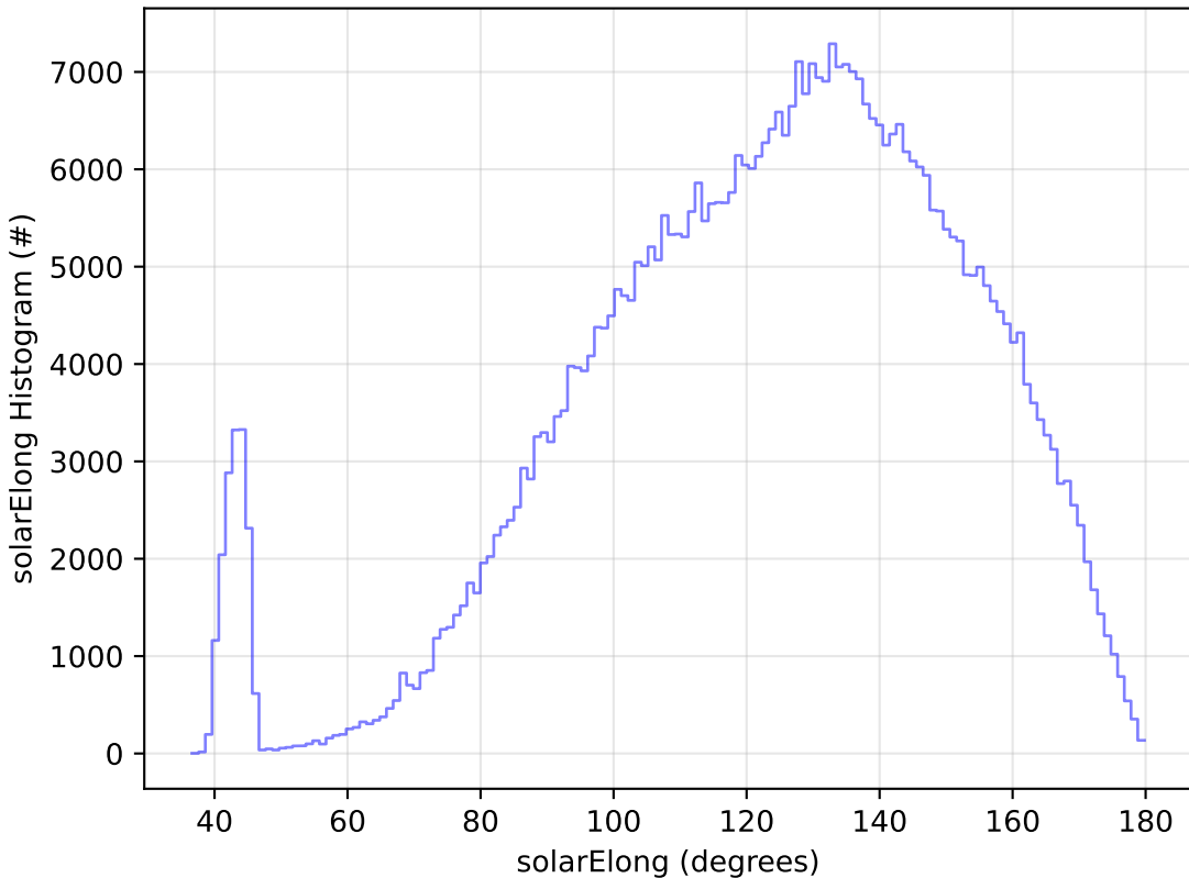
too_5_4v3.4_10yrs All sky r band: solarElong Histogram
