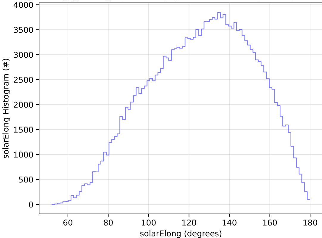
too_5_4v3.4_10yrs All sky g band: solarElong Histogram
