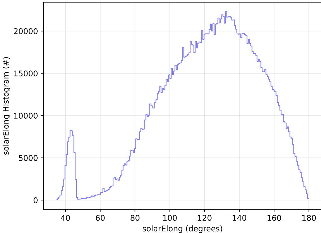
too_5_4v3.4_10yrs All sky all bands: solarElong Histogram
