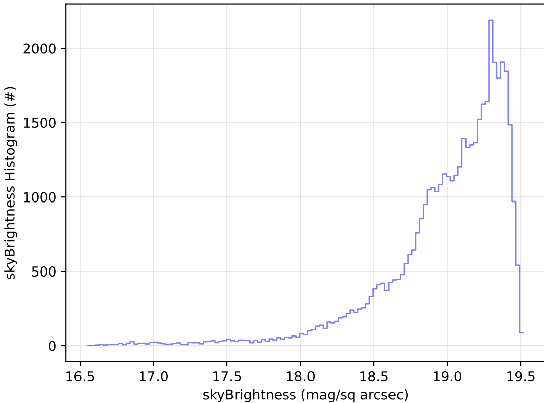
too_5_4v3.4_10yrs Yr 1 z band: skyBrightness Histogram
