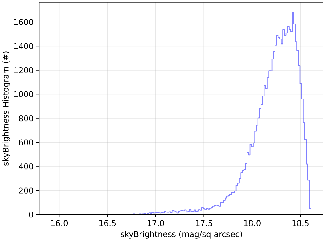
too_5_4v3.4_10yrs Yr 1 y band: skyBrightness Histogram
