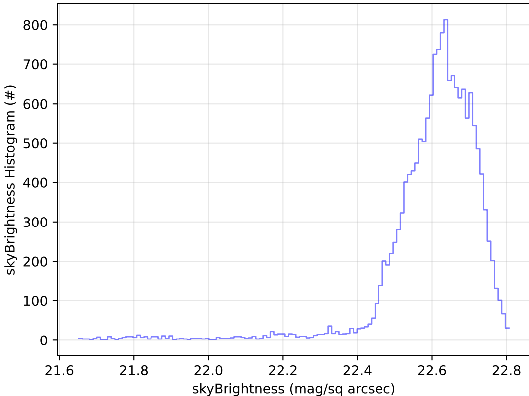
too_5_4v3.4_10yrs Yr 1 u band: skyBrightness Histogram
