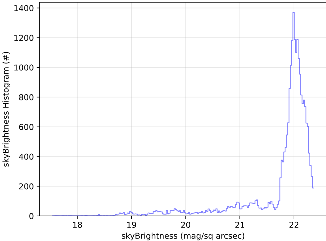
too_5_4v3.4_10yrs Yr 1 g band: skyBrightness Histogram
