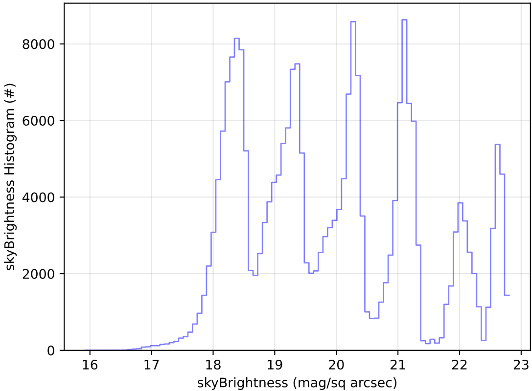
too_5_4v3.4_10yrs Yr 1 all bands: skyBrightness Histogram
