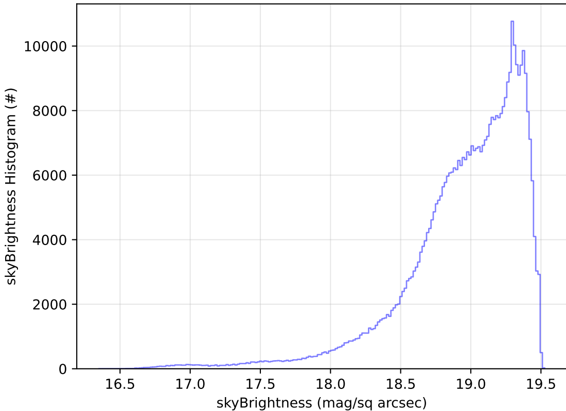
too_5_4v3.4_10yrs WFD z band: skyBrightness Histogram
