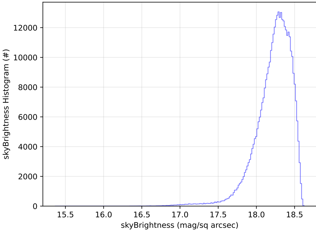
too_5_4v3.4_10yrs WFD y band: skyBrightness Histogram
