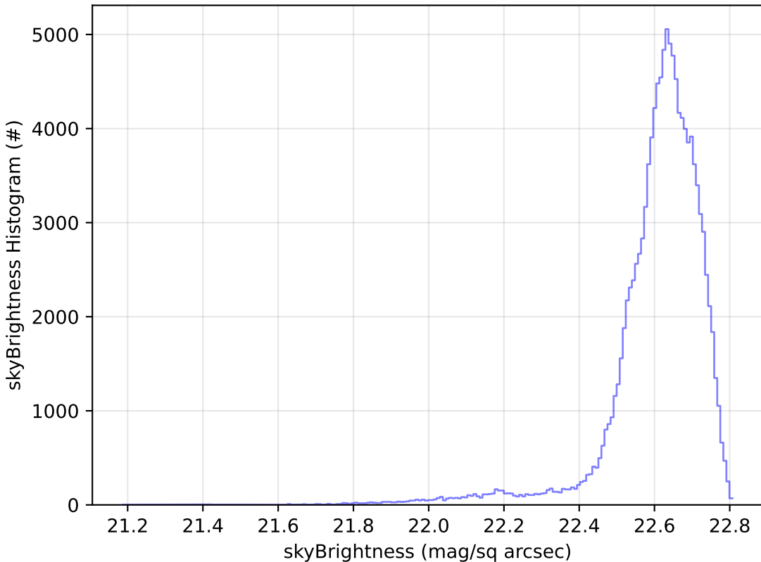
too_5_4v3.4_10yrs WFD u band: skyBrightness Histogram
