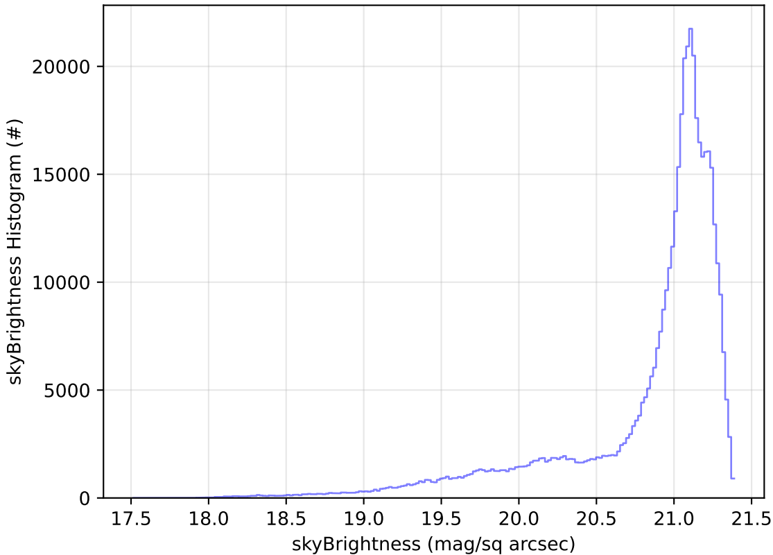
too_5_4v3.4_10yrs WFD r band: skyBrightness Histogram
