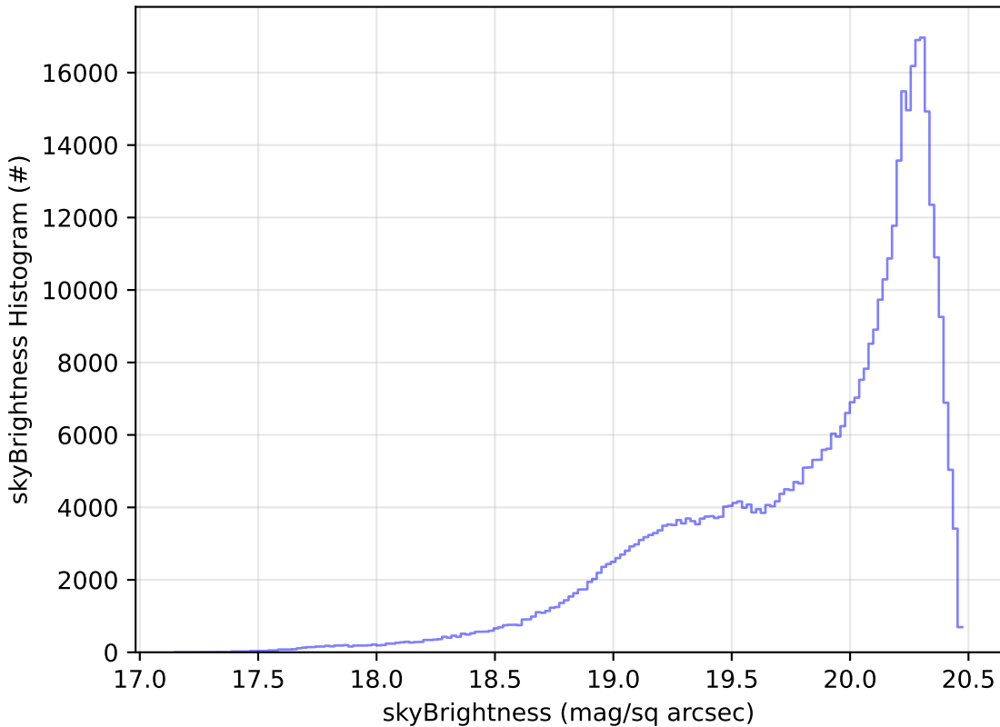
too_5_4v3.4_10yrs WFD i band: skyBrightness Histogram
