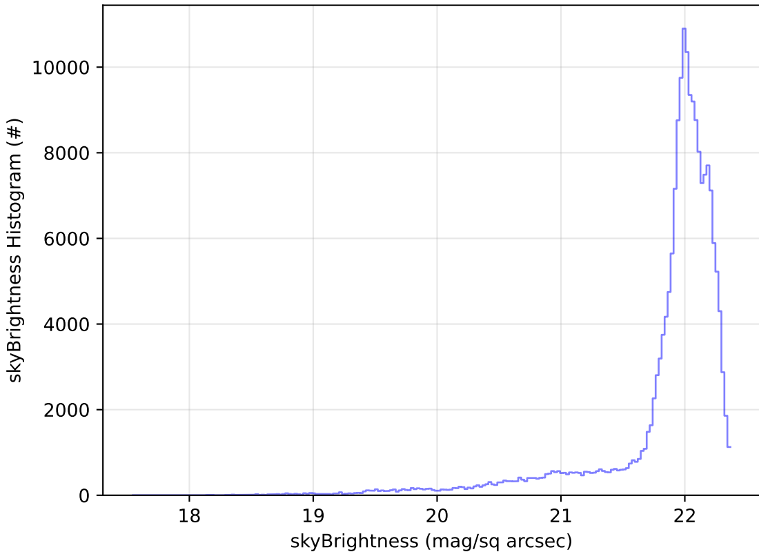
too_5_4v3.4_10yrs WFD g band: skyBrightness Histogram
