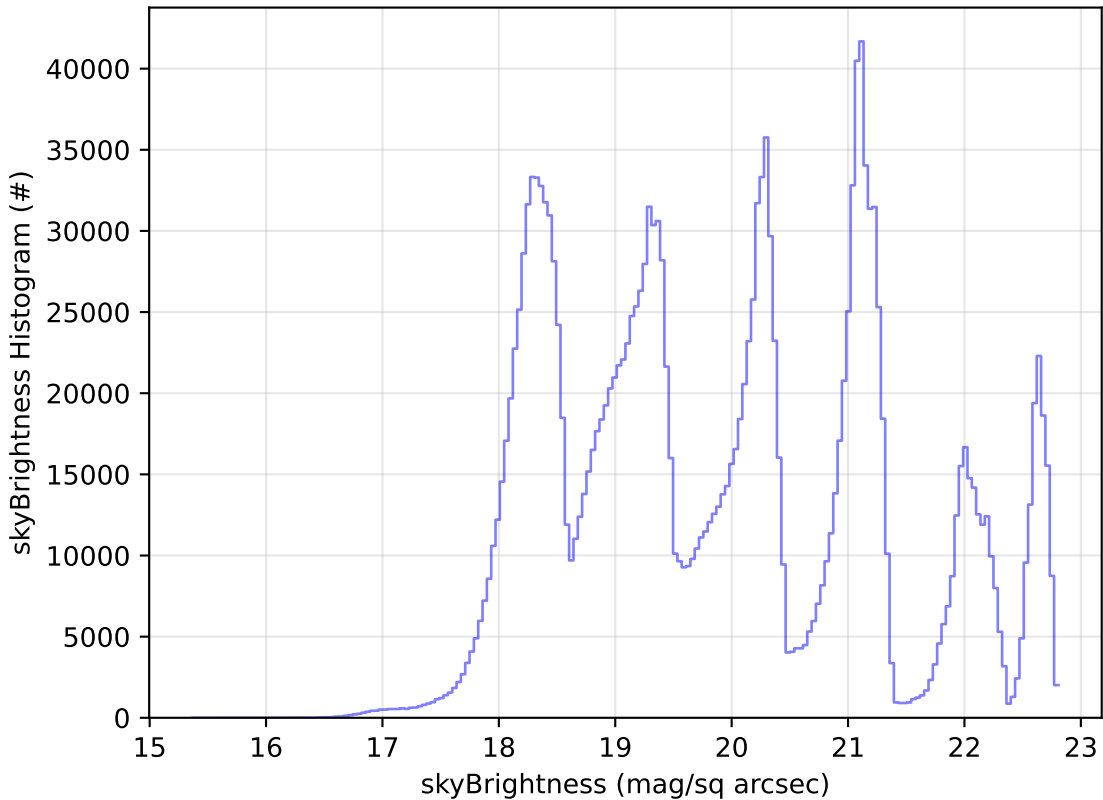
too_5_4v3.4_10yrs WFD all bands: skyBrightness Histogram
